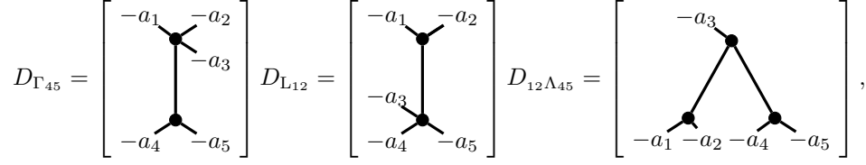
FIGURE 3. Level graphs of boundary divisors for strata \Omega\mathcal{M}_{0,5}(a_1, \dots, a_5)
